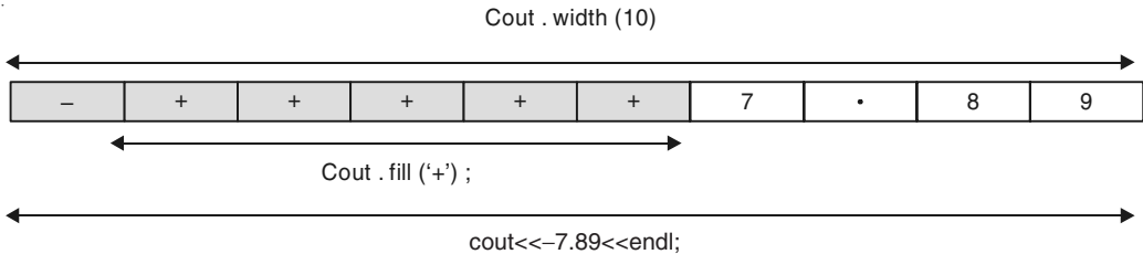
Figure 11.9. Implementation of flags used in C++
